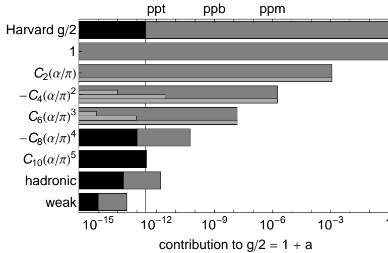
Fig. 8.2. Contributions to g/2 for the experiment (top bar), terms in the QED series (below), and from small distance physics (below). Uncertainties are black. The inset light gray bars represent the magnitude of the larger mass-independent terms ( A_1 ) and the smaller A_2 terms that depend upon either m_e/m_\mu or m_e/m_\tau . The even smaller A_3 terms, functions of both mass ratios, are not visible on this scale.
