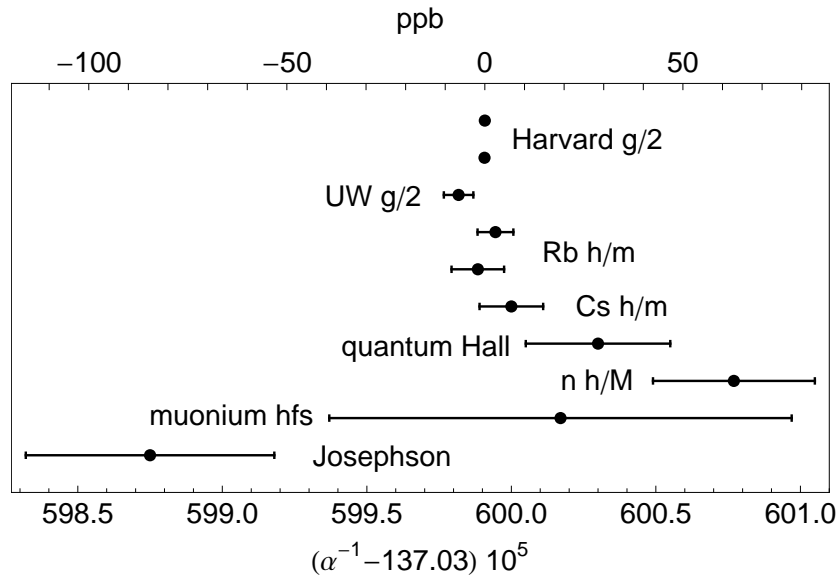
Fig. 8.5. Less accurate measurements of \alpha compared upon an expanded scale. The uncertainties in the two most accurate determinations of \alpha are too small to be visible on this large scale.
