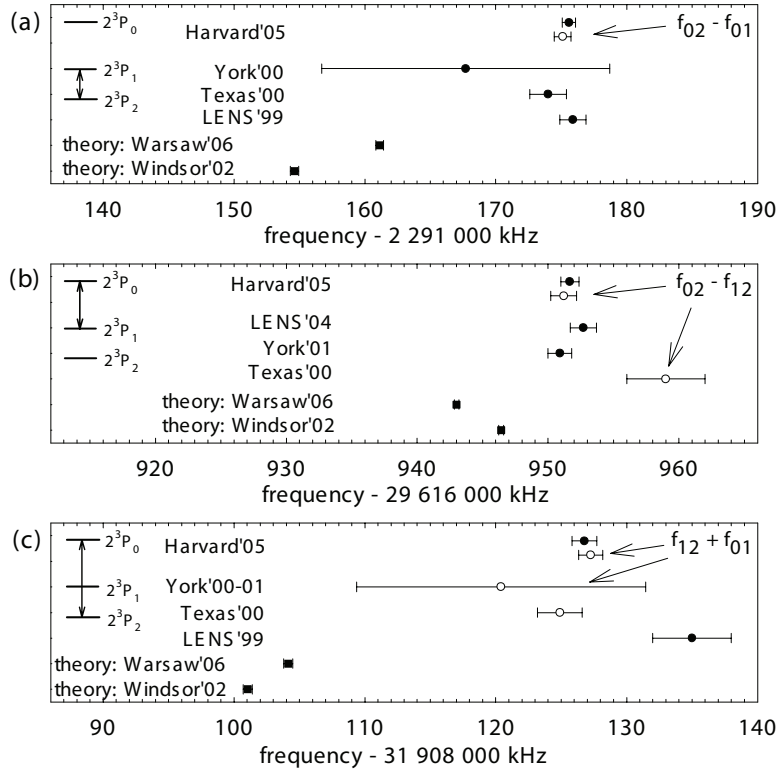
Fig. 8.4. Most accurate measured [1–4] and calculated [5, 6] ^4\text{He} fine structure intervals with standard deviations. Directly measured intervals (black filled circles) are compared to indirect values (open circles) deduced from measurements of the other two intervals. Uncorrelated errors are assumed for the indirect values for other groups.
