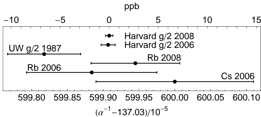
Fig. 8.1. The most precise determinations of \alpha .
