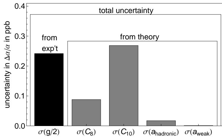
Fig. 8.3. Experimental uncertainty (black) and theoretical uncertainties (gray) that determine the uncertainty in the \alpha that is determined from the measured electron g/2
