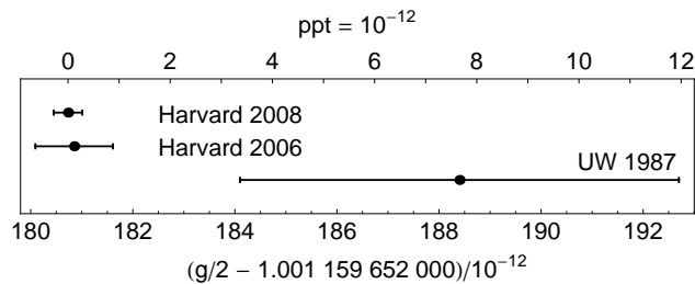
Fig. 6.1. Most accurate measurements of the electron g/2 .
