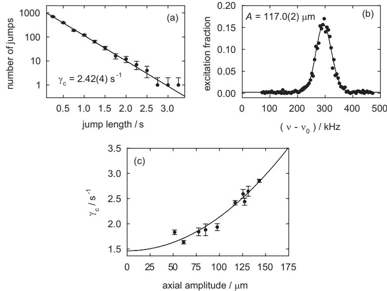
Fig. 6.9. Measurement of the cyclotron damping rate at 146.70 GHz, near the upper sideband of TE 136 . The cyclotron damping rate as a function of axial amplitude (c) extrapolates to the desired lifetime. Each point in (c) consists of a damping rate measured from a fit to a histogram of cyclotron jump lengths (a) as well as an axial amplitude measured from a driven cyclotron line (b).
