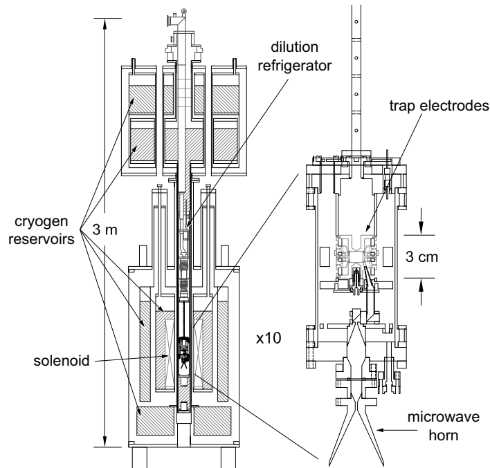
Fig. 6.4. The apparatus includes a trap electrodes near the central axis, surrounded by a superconducting solenoid. The trap is suspended from a dilution refrigerator.
