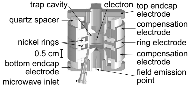
Fig. 6.3. Cylindrical Penning trap cavity used to confine a single electron and inhibit spontaneous emission.
