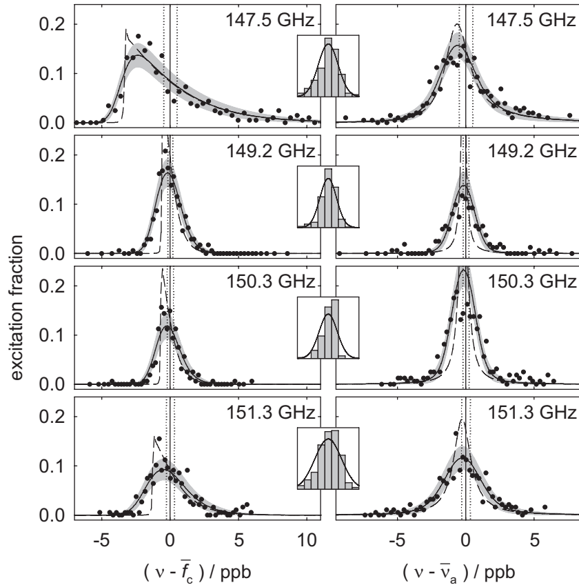
Fig. 6.7. Quantum-jump spectroscopy lineshapes for cyclotron (left) and anomaly (right) transitions with maximum-likelihood fits to broadened lineshape models (solid) and inset resolution functions (solid) and edge-tracking data (histogram). Vertical lines show the 1\text{-}\sigma uncertainties for extracted resonance frequencies. Corresponding unbroadened lineshapes are dashed. Gray bands indicate 1\text{-}\sigma confidence limits for distributions about broadened fits. All plots share the same relative frequency scale.
