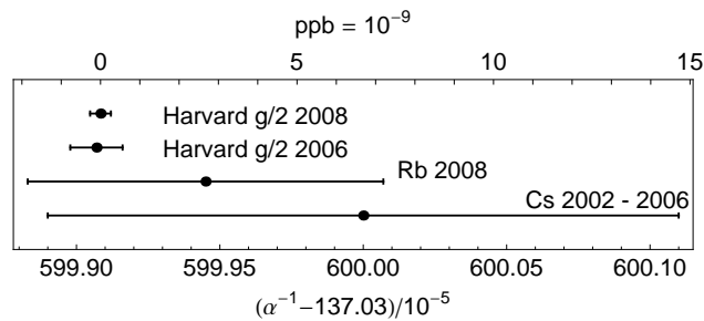
Fig. 6.11. The most accurate determinations of \alpha are determined from the measured electron g/2 . These are compared to the best independently measured values.
