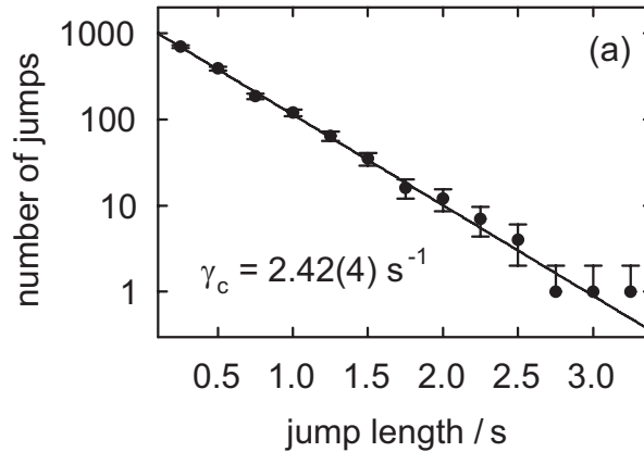
Fig. 6.6. A histogram of the time that the electron spends in the first excited state that is fit to an exponential reveals the substantial inhibition of the spontaneous emission of synchrotron radiation. The decay time, 0.41s in this example, depends on how close the cyclotron frequency is to neighboring radiation modes of the trap cavity. Lifetimes as long as 16 s have been observed.
