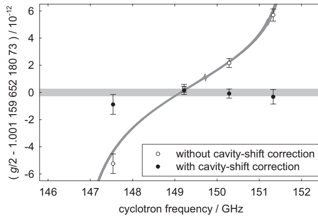
Fig. 6.10. Four measurements of g/2 without (open) and with (filled) cavity-shift corrections. The light gray uncertainty band shows the average of the corrected data. The dark gray band indicates the expected location of the uncorrected data given our result in Eq. 6.23 and including only the cavity-shift uncertainty.
