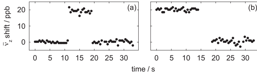
Fig. 6.5. Two quantum jumps: A cyclotron jump (a) and spin flip (b) measured via a QND coupling to shifts in the axial frequency.
