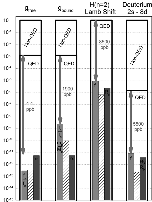
Fig. 6.12. Comparisons of precise tests of QED. The arrows represent the fractional accuracy to which the QED contribution to the measured g values and frequencies that are measured.
