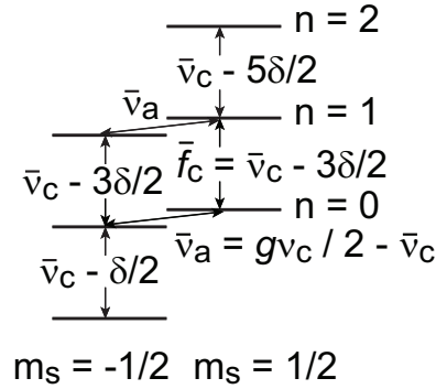
Fig. 6.2. Lowest cyclotron and spin levels of an electron in a Penning trap.
